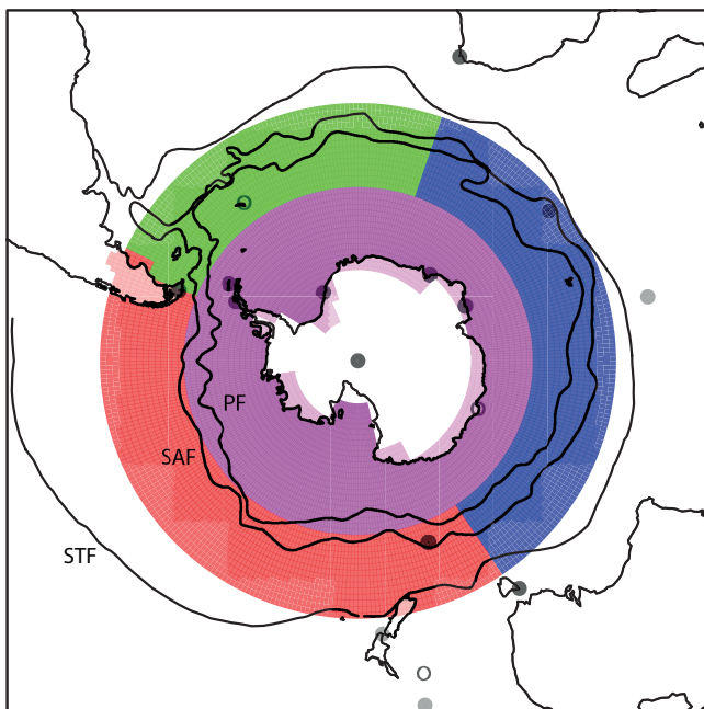
Fig. 1. Subregions of the Southern Ocean (44° S to 75° S) used in this paper are the circular region 44–58° S (green, red and blue combined) and the major ocean basins (Pacific, Indian and Atlantic) in this band, and the circumpolar region from 58° S–75° S (purple). Overlain is the network of atmospheric observations of CO 2 . The colour of the dot indicates how many inversions used data from that location (black: all or almost all inversions, grey: around half the inversions, white: one or two inversions). We note that the temporal period over which the data was collected is not the same in all the stations. Overlain on these figures, from north to south are the mean positions of the major fronts Subtropical Front (STF), Subantarctic Front (SAF) and the Polar Front (PF) following Orsi et al. (1995).
