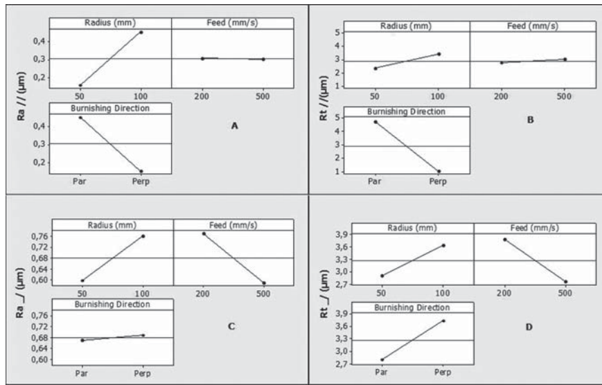
FIGURE 6.—Summary graph of the influence of experimental parameters on the index of measured surface roughness in convex steel G10380 workpieces: (A) Ra // , (B) Rt // , (C) Ra \perp , and (D) Rt \perp .
