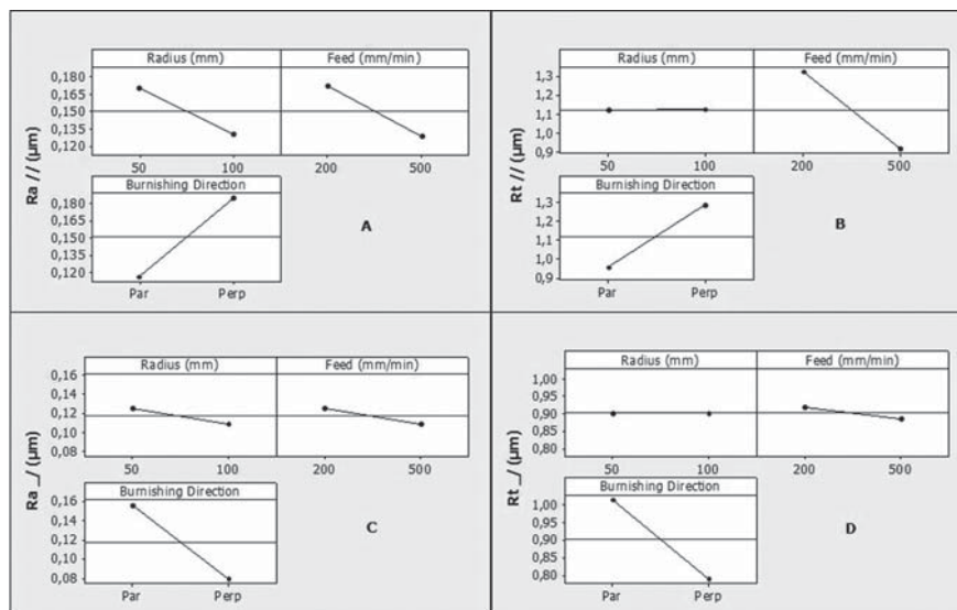
FIGURE 7.—Summary graph of the influence of experimental parameters on the index of measured surface roughness in concave aluminium A92017 workpieces: (A) Ra // , (B) Rt // , (C) Ra \perp , and (D) Rt \perp .
