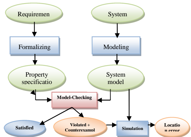
Figure 3. The model checking approach.
