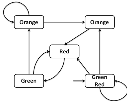
Figure 4. An example of Kripke structure: a traffic light.
