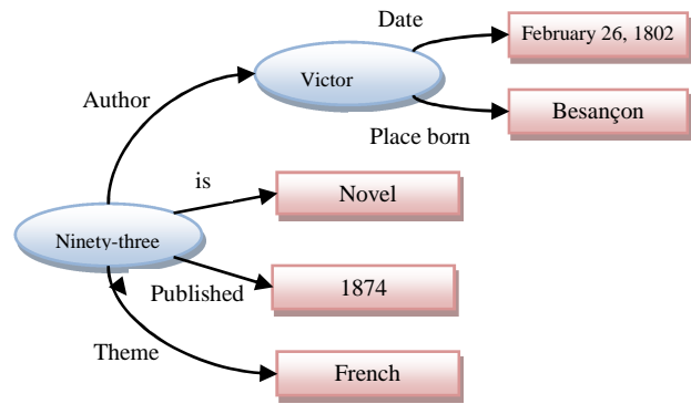
Figure 9. Example of an RDF graph.
