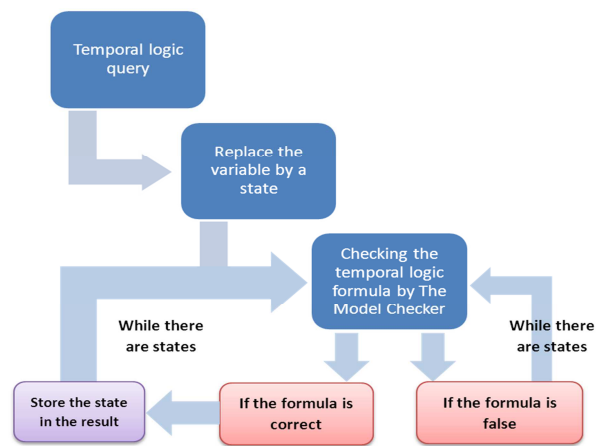
Figure 8. The STL Resolver tool.
