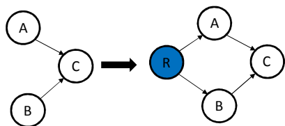
Figure 6. A root is a single node that has no predecessor. In this graph, we have a node A and a node B, two roots, and then we will create a new virtual root (blue circle "R") that points to the two roots.
