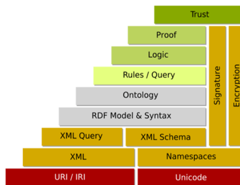
Figure 1. Stack of languages of the Semantic Web. [2]
