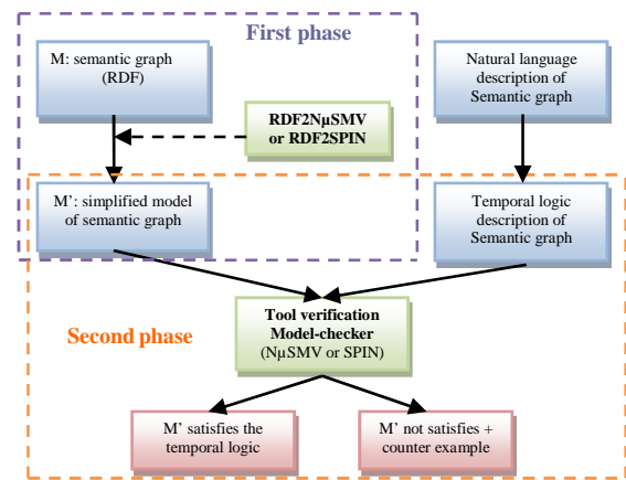
Figure 5. The ScaleSem architecture.
