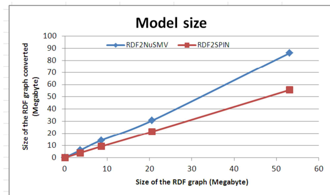
Figure 11. Size of the models.
