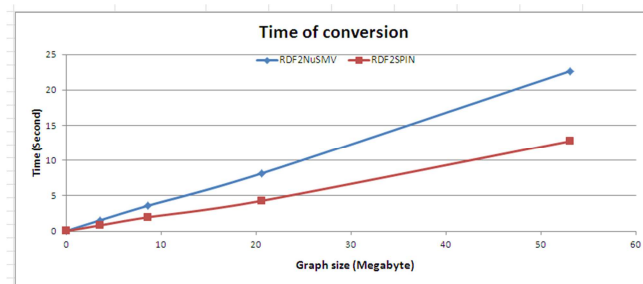
Figure 10. Time of conversion of Semantic graphs.
