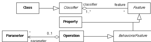
Fig. 3. Class diagram from the Veha metamodel: Features of a Classifier.
