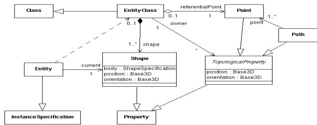
Fig. 4. Class diagram from the Veha metamodel: EntityClass.
