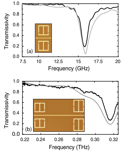
FIG. 3. Simulated (gray curves) and experimental (black curves) transmissivity of (a) the GHz MMs and (b) the THz MMs on the PGL. The two insets are optical images of single-pair (top) and dual-pair (bottom) THz metamaterial elements adjacent to the PGL.
