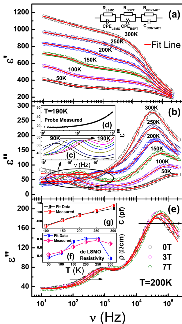
FIG. 1. (Color online) The (a) real part ( \epsilon' ) and (b) imaginary part ( \epsilon'' ) of permittivity as function of frequency for BSPT/LSMO heterostructure at various temperatures. The inset shows the CPE equivalent circuit. Solid lines: overall response fitted by equivalent circuit; (c) frequency-dependent of \epsilon'' in low-frequency region from 90 to 190 K; (d) the dielectric spectrum with probe contact at 190 K; (e) the relaxation characteristic under magnetic field at 200 K; (f) dc resistivity characteristic of LSMO; and (g) capacitance of BSPT/LSMO for fitting and measured data at elevated temperature.
