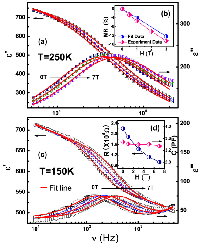
FIG. 2. (Color online) (a) Frequency and magnetic field dependence of dielectric behavior measured from 10 000 to 200 000 Hz at 250 K; (b) the magnetic field variation in MR for fitting and experiment data, respectively; (c) the dielectric behavior under magnetic field in low-frequency region at 150 K; (d) variation of the fitted resistance and capacitance under magnetic field.
