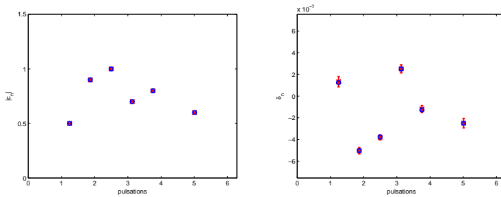
FIG. 3.2. Estimation results in the case of 6 cisoids ( SNR = 23.27 dB): complex values of (|c_n|)_{1 \leq n \leq N} (left); real values of frequency perturbations (\delta_n)_{1 \leq n \leq N} as a function of (\theta_n)_{1 \leq n \leq N} (right). The exact values are depicted with blue circles and the confidence intervals on the estimates in red (the mean is indicated by a cross).
