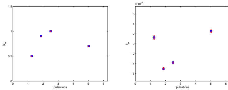
FIG. 3.1. Estimation results in the case of 4 cisoids ( SNR = 19.82 dB): complex values of (|c_n|)_{1 \leq n \leq N} (left); real values of frequency perturbations (\delta_n)_{1 \leq n \leq N} as a function of (\theta_n)_{1 \leq n \leq N} (right). The exact values are depicted with blue circles and the confidence intervals on the estimates in red (the mean is indicated by a cross).
