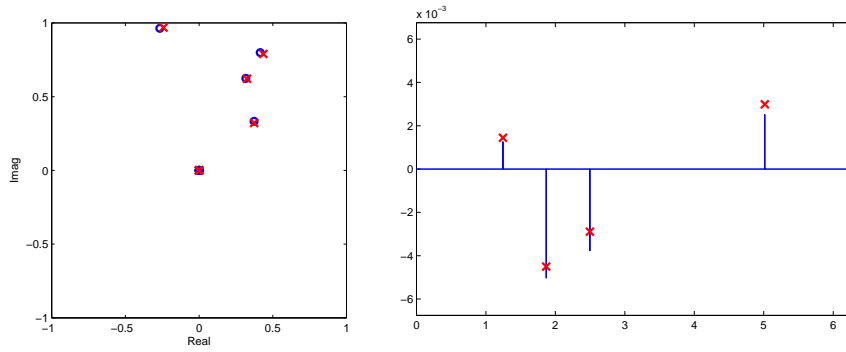
FIG. 3.1. Estimation results in the case of 4 cisoids ( SNR = 20.06 dB): Exact (circles) and estimated (crosses) complex values of (c_n)_{1 \leq n \leq N} (left); Exact (continuous) and estimated (crosses) real values of frequency perturbations (\delta_n)_{1 \leq n \leq N} as a function of (\theta_n)_{1 \leq n \leq N} (right).
