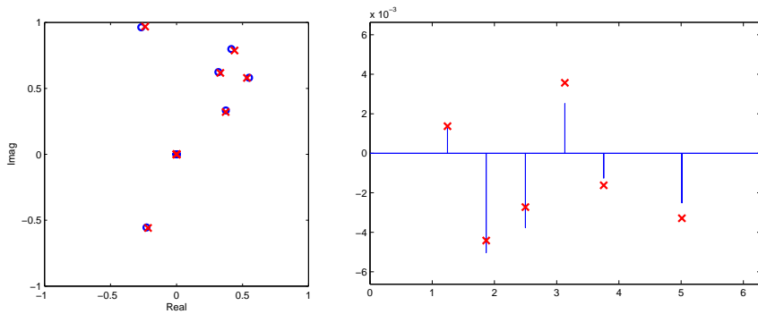
FIG. 3.2. Estimation results in the case of 6 cisoids ( SNR = 18.43 dB): Exact (circles) and estimated (crosses) complex values of (c_n)_{1 \leq n \leq N} (left); Exact (continuous) and estimated (crosses) real values of frequency perturbations (\delta_n)_{1 \leq n \leq N} as a function of (\theta_n)_{1 \leq n \leq N} (right).
