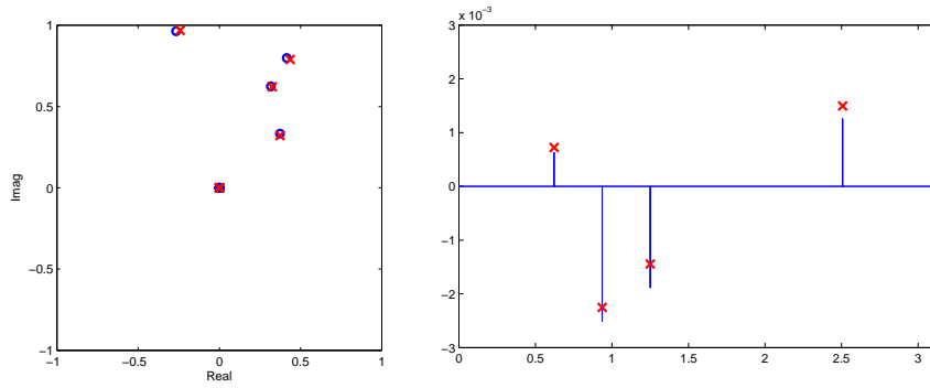
FIG. 3.1. Estimation results in the case of 4 cisoids (SNR = 20.06 dB): Exact (circles) and estimated (crosses) complex values of (c_n)_{1 \leq n \leq N} (left); Exact (continuous) and estimated (crosses) real values of frequency perturbations (\delta_n)_{1 \leq n \leq N} as a function of (\theta_n)_{1 \leq n \leq N} (right).
