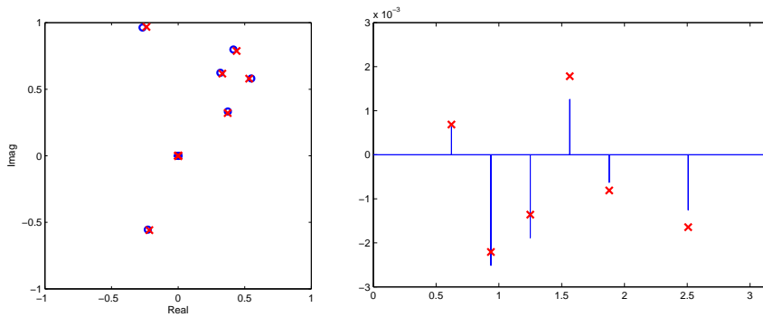
FIG. 3.2. Estimation results in the case of 6 cisoids (SNR = 20.06 dB): Exact (circles) and estimated (crosses) complex values of (c_n)_{1 \leq n \leq N} (left); Exact (continuous) and estimated (crosses) real values of frequency perturbations (\delta_n)_{1 \leq n \leq N} as a function of (\theta_n)_{1 \leq n \leq N} (right).
