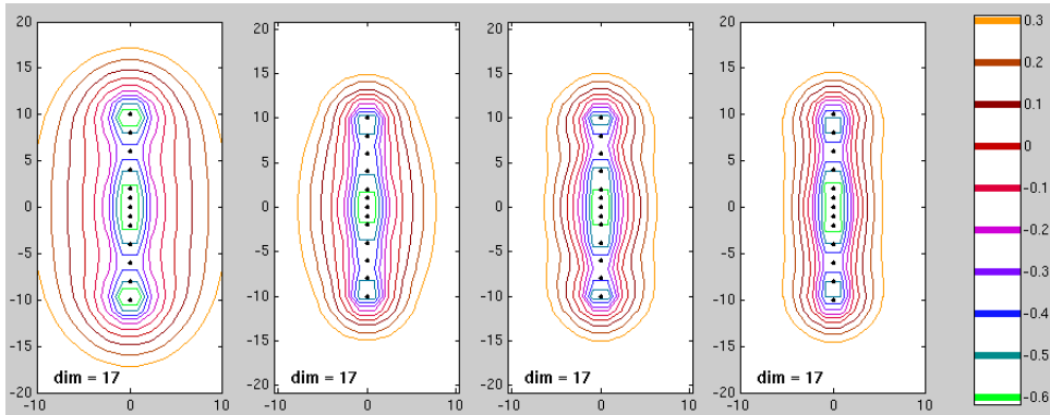
Figure 3: The pseudospectra of the state transition matrix A for the four solutions corresponding to n = 5 .
