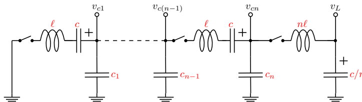
Figure 1: The passive circuit used as a Marx generator.
