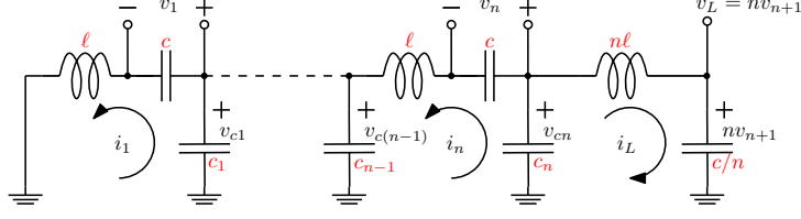
Figure 4: Sign conventions in the models of the Marx generator circuit.
