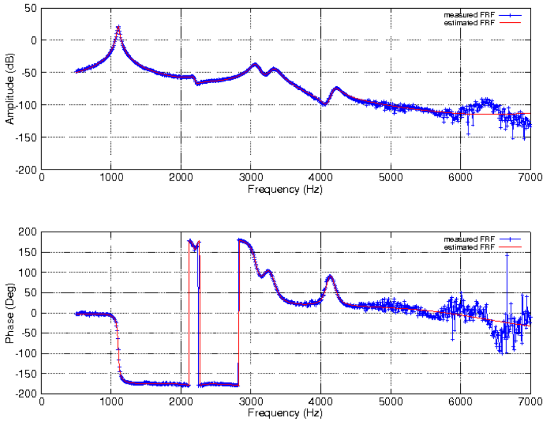
Figure 12: Example of compliance measurement without the use of artificial lip. View of the measured data (+) and the estimated data (-) using the least mean square method.
