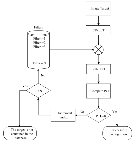
Fig. 5. Face recognition algorithm
