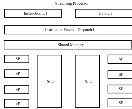
Fig. 2. GPU Architecture
