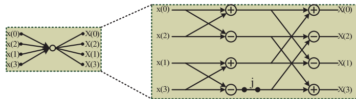
Fig. 1. Radix-4 butterfly
