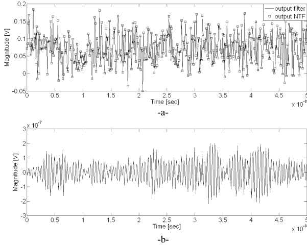
Figure 5. Comparison between desired and estimated output in time-domain
