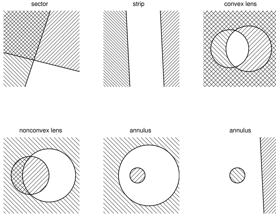
FIGURE 107.1 Six different configurations (in white) of intersections of two disks of the Riemann sphere.
