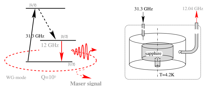
Fig. 1. Principle of the whispering gallery mode maser oscillator.
