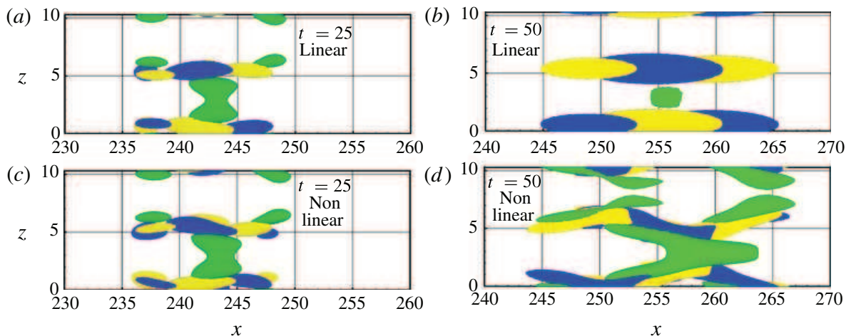
FIGURE 16. (Colour online) Isosurfaces of the perturbation obtained at t = 25 (a,c) and t = 50 (b,d), for a linear simulation (a,b) and a complete nonlinear simulation (c,d). The grey (green online) surfaces indicate the negative streamwise component of the perturbation velocity ( u' = -0.05 for t = 25 and u' = -0.08 for t = 50 ), the dark and light (blue and yellow online) surfaces indicate negative and positive streamwise vorticity, respectively ( \omega'_x = \pm 0.15 for t = 25 and \omega'_x = \pm 0.2 for t = 50 ).
