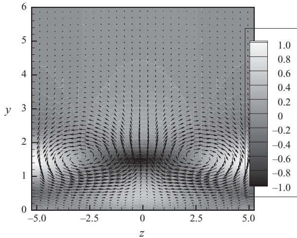
FIGURE 1. Optimal initial perturbation on the x=450 plane computed for the target time t = T_{max} and Re = 610 . The vectors represent the v and w components, whereas the shading is relative to the normalized streamwise velocity.
