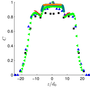
Figure 4. Variation of objects contrast with normalized distance from the focal plane
