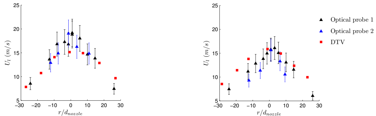
Figure 13. Comparison of liquid velocity (magnitude) at 780 (left) and at 890 (right) nozzle diameters from the nozzle exit; the first two datasets corresponds to optical probe measurements (respectively on a horizontal then a vertical jet diameter), the last dataset is obtained by our imaging method
