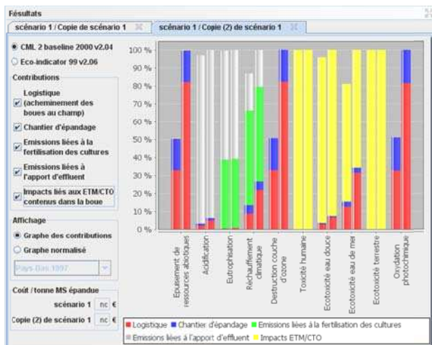
CML Baseline 2000
