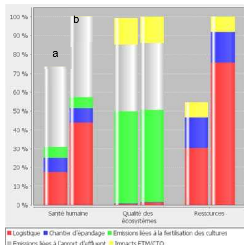
Ecoindicator 99
