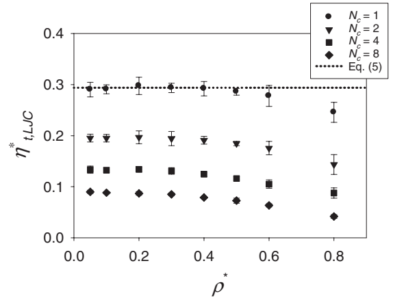
FIG. 1. Translational viscosity of the fully flexible LJC fluid versus density for different chain lengths ( N_c = 1, 2, 4 , and 8 ) and for T^* = 3 . The dotted line corresponds to the zero-density viscosity of the monomer.
