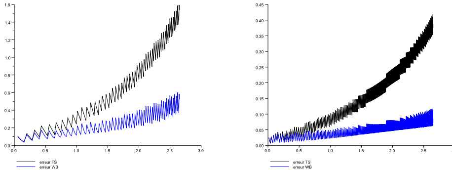
Fig. 5. Time evolution of L^1 error for a N -wave solving (69) with different grids.
