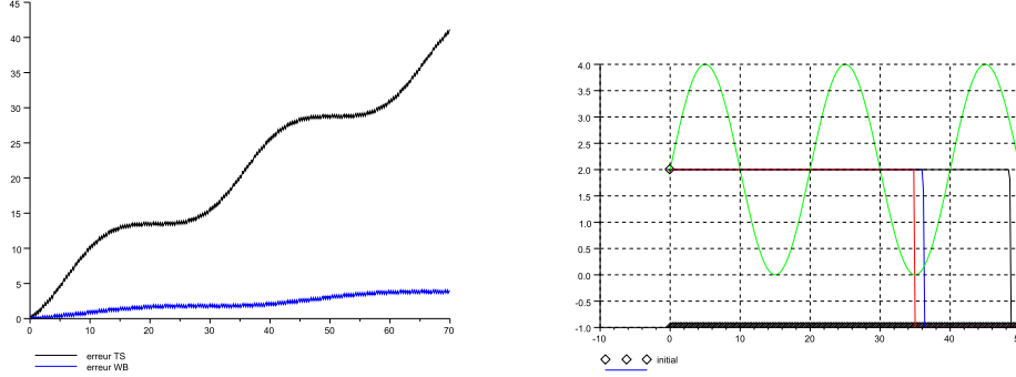
Fig. 6. Time evolution of L^1 error for a "speedup" Riccati source term.
