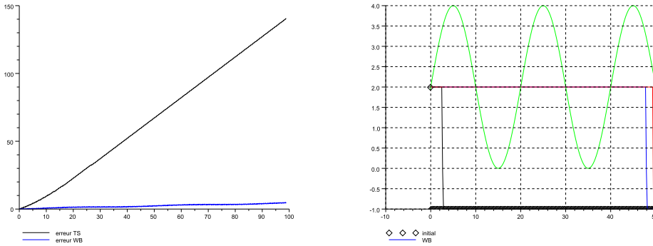
Fig. 7. Time evolution of L^1 error for a "slowdown" Riccati source term.
