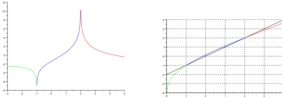
Fig. 8. Illustration of the functions \phi(u) and w(u, a) for the equation (70).
