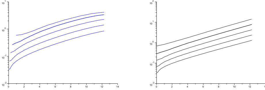
Fig. 3. Time evolution of the measured L^1 error for (5) with \Delta x = 2^{-n} , n = 0, 1, 2, 3, 4 . The WB scheme (left) shows a weaker dependence on the grid compared to the TS one (right) which displays a neat exponential growth.
