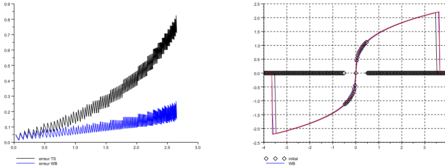
Fig. 4. Time evolution of L^1 error for a N -wave solving (69).
