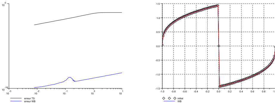
Fig. 9. Time evolution of L^1 error for the static roll-wave.
