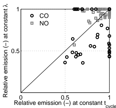
Figure 13: Relative CO and NO emissions (-) at constant t_{\text{cycle}} and \lambda , for all burner configurations in parallel firing mode.
