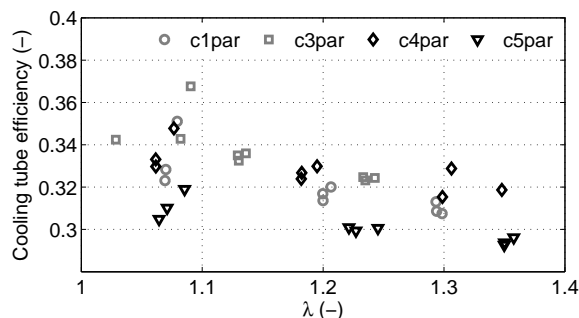
Figure 7: Cooling tube efficiency (-) versus \lambda (-) for parallel firing mode and all burner configurations and cycle times.
