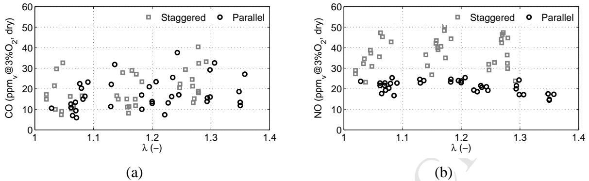
Figure 4: (a) CO and (b) NO emissions ( \text{ppm}_v @ 3\% \text{O}_2, \text{dry} ) for the different firing modes for all burner configurations, values of \lambda and cycle times.
