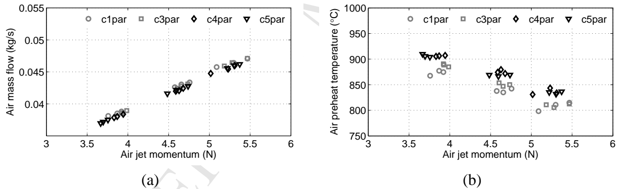
Figure 9: Correlation between the combustion air jet momentum (N) and (a) the mass flow (kg/s) and (b) the preheat temperature ( ^{\circ}\text{C} ) of the combustion air for all configurations firing parallel mode and all values of \lambda and cycle time.
