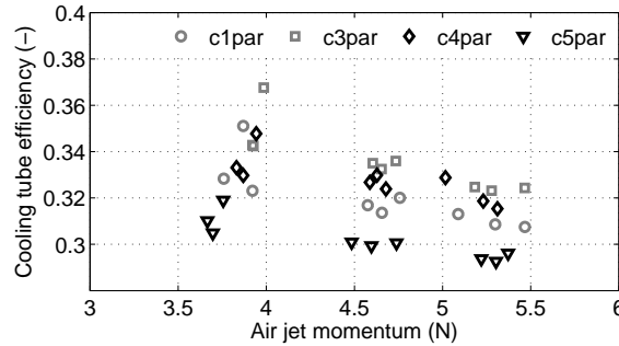
Figure 10: Cooling tube efficiency (-) versus air jet momentum (N) for all configurations firing parallel mode and all values of \lambda and cycle time.
