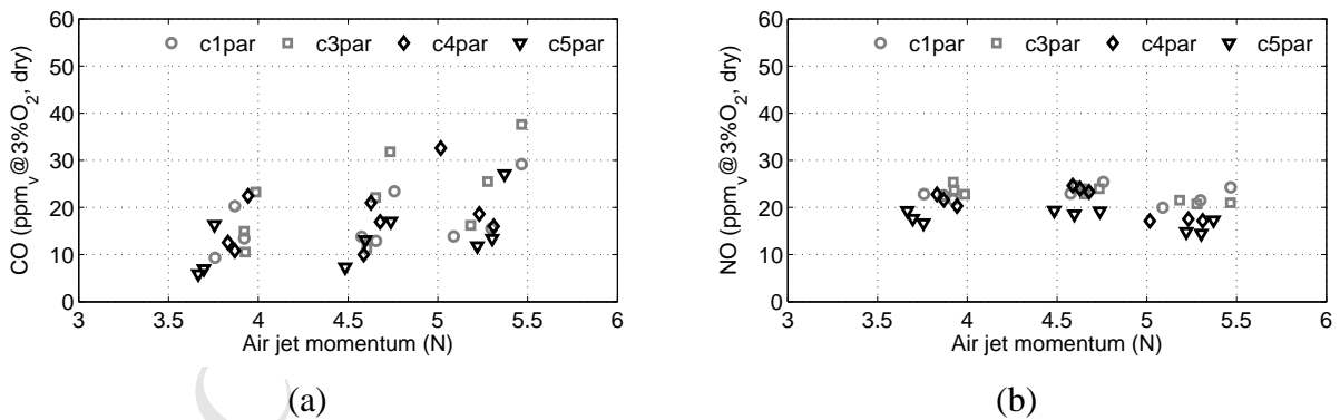
Figure 11: (a) CO and (b) NO emissions ( \text{ppm}_v @ 3\% \text{O}_2, \text{dry} ) versus combustion air jet momentum (N) for all configurations firing parallel mode and all values of \lambda and cycle time.
