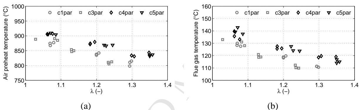
Figure 6: (a) Combustion air preheat temperatures and (b) regenerated flue gas exit temperature ( ^{\circ}\text{C} ) for parallel firing mode and all values of \lambda and t_{\text{cycle}} .
