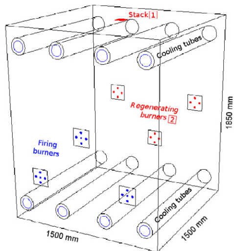
Figure 1: Furnace sketch. The boxed numbers 1 and 2 indicate the two sample positions for the flue gas. Sampling point 2 is after the regenerators. All dimensions are in mm. The sketch represents burner configuration C5 firing in parallel mode (see also Table 1).
