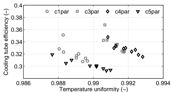
Figure 14: Cooling tube efficiency (-) versus temperature uniformity (-) for all burner configurations in parallel firing mode and all values for \lambda and cycle time.
