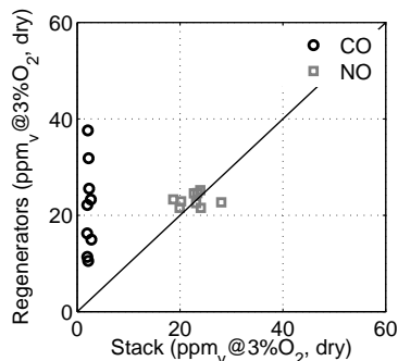
Figure 2: Emission measurements ( \text{ppm}_v @ 3\% \text{O}_2, \text{dry} ) in the flue gas from the stack and from the regenerators for burner configuration C3 firing in parallel mode.
