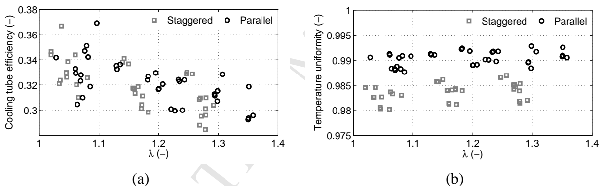
Figure 3: (a) Cooling tube efficiency (-) and (b) temperature uniformity (-) for the different firing modes for all burner configurations, values of \lambda and cycle times.
