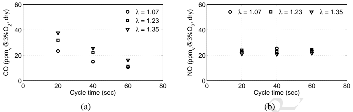
Figure 8: (a) CO and (b) NO emissions ( \text{ppm}_v @ 3\% \text{O}_2 , dry) versus the cycle time for C3 configuration in parallel firing mode, for all values of \lambda .
