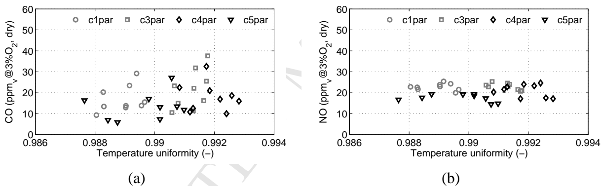
Figure 15: (a) CO and (b) NO emissions ( \text{ppm}_v @ 3\% \text{O}_2, \text{dry} ) versus the temperature uniformity (-) for all burner configurations in parallel firing mode and all cycle times and values for \lambda .
