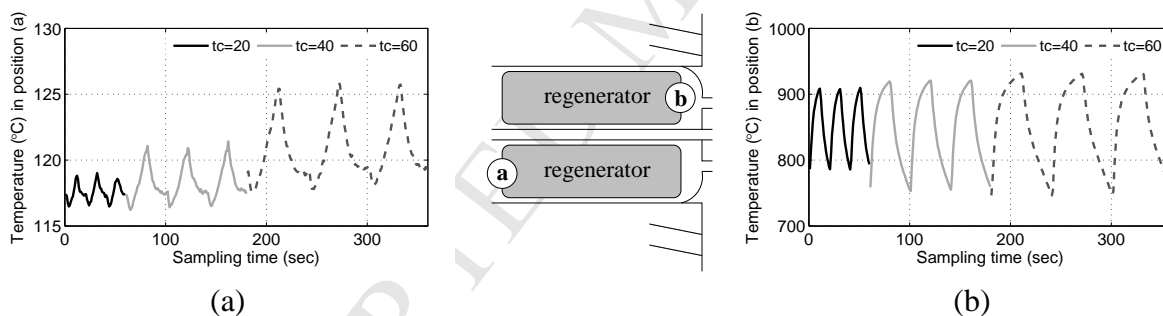
Figure 12: Temperature (°C) at the cold side, position (a), and at the hot side, position (b), of the regenerator of one burner during configuration C3, parallel firing mode, \lambda = 1.2 and all cycle times. The actual measurement positions of Figures (a) and (b) are represented in the sketch of the burner by the encircled a and b, respectively. For every cycle time three entire cycles are presented, with the first half of the cycle a regenerating period.
