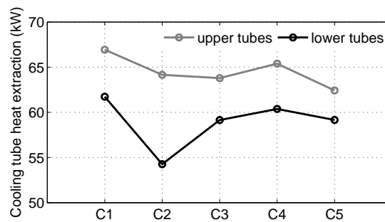
Figure 5: Cooling tube heat extraction ( \text{kW}_{\text{th}} ) versus all burner configurations for parallel firing mode, \lambda = 1.1 and t_{\text{cycle}} = 20 \text{ sec} .
