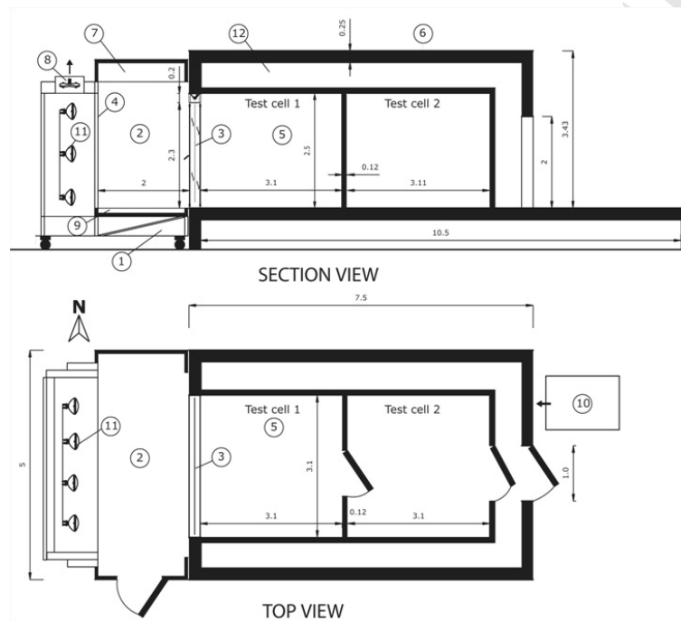
Figure 8: Test cell facility scheme: 1, cooling unit; 2, weather generator; 3, double skin façade; 4, protection glass of the solar simulator; 5, test cell; 6, concrete; 7, air blowing plenum; 8, solar simulator's heat removal ventilators; 9, air extraction plenum; 10, HVAC unit of the buffer zone; 11, solar simulator; 12, controlled buffer zone. (Metric units) [16].
