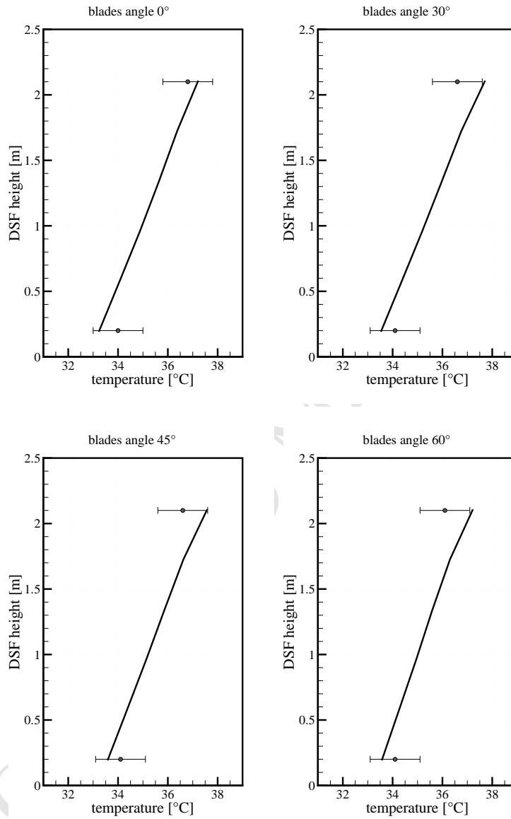
Figure 11: Air temperature profile in the right channel of the DSF for an airflow equal to 400\text{m}^3\text{h}^{-1} - circle: experimental data and line: numerical modelling.
