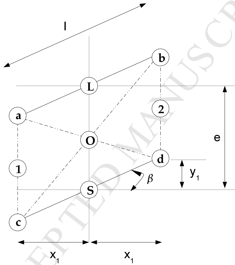
Figure 4: Hottel method applied to the double skin façade: e = 0.025m spacing between the blinds, l = 0.025m blind's width and \beta blind's angle.
