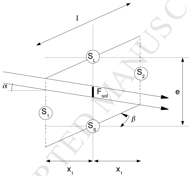
Figure 5: Schematic of different surfaces considered for the calculation of the irradiation in short wavelength.
