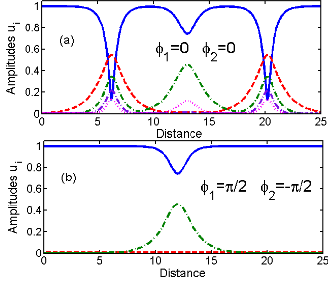
Fig. 2 : Evolution with distance z of the amplitudes of the pump and its harmonics u_i : (a) initial in-phase and parallel modulation, CW pump (blue solid curve), the sideband at frequency shift \Omega=+\Omega_l from the pump (red dashed curve), its second harmonic at \Omega=+2\Omega_l (green dot-dashed curve), third harmonic \Omega=+3\Omega_l (violet dot-dashed curve), and fourth harmonic \Omega=+4\Omega_l (pink dotted curve) corresponding to the case in Fig.1; (b) initial modulation orthogonal to the pump.
