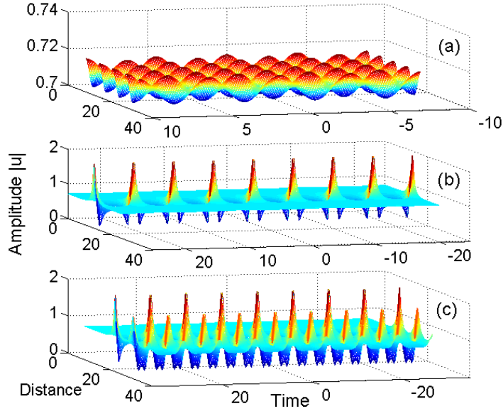
Fig. 4: Surface plot of the amplitude |u| with orthogonal input pump and sidebands \phi_u=0 , \phi_v=\pi , and the different sideband modulation frequencies: (a) \Omega=\sqrt{2} , (b) \Omega=0.5 and (c) \Omega=0.4 .
