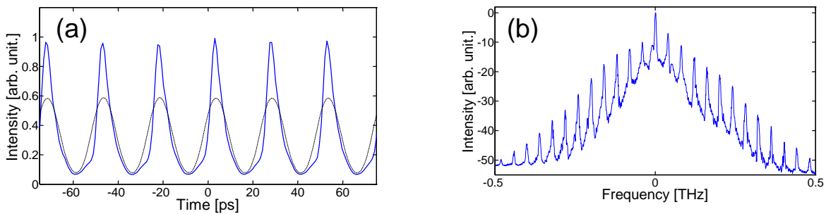
Fig. 10 : (a) Temporal profiles at the input (dashed line) and output (solid line) of the fiber when pump and signal waves have parallel polarization states (b) Experimental spectrum at the output of the fiber for input parallel polarized pump and signal and for a pump power of 19.7 dBm. Note that the output polarizer was oriented parallel to the pump polarization.
