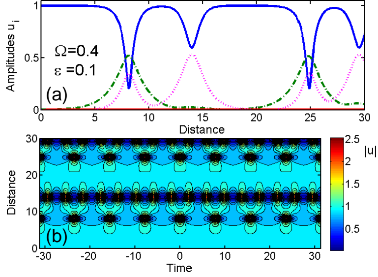
Fig. 8 : CW and sideband (a) amplitudes and (b) contour plot in the u mode with \Omega=0.4 , \varepsilon_u=0 , \varepsilon_v=10^{-1} , \phi_u=\phi_v=0 .
