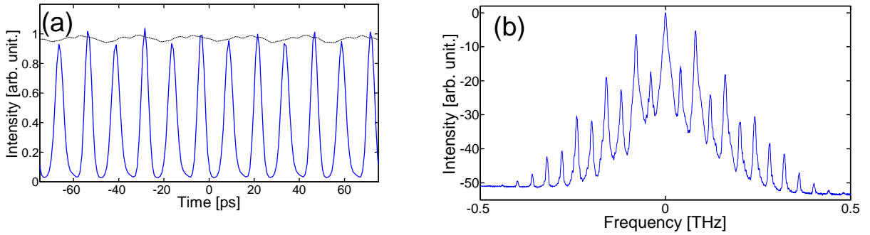
Fig. 11 : (a) Experimental temporal profiles at the input (dashed line) and output (solid line) of the fiber for orthogonal polarized pump and signal waves. (b) Corresponding output experimental spectrum. The output polarizer was oriented parallel to the pump polarization.
