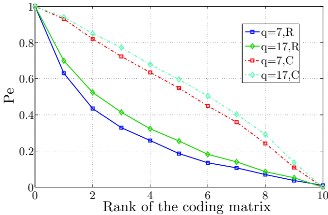
Fig. 4. Proportion of erroneously reconstructed quantized samples as a function of the rank of A sink for q = 7 and q = 17 , with the proposed approach (R) and with a conventional Gaussian elimination (C)
