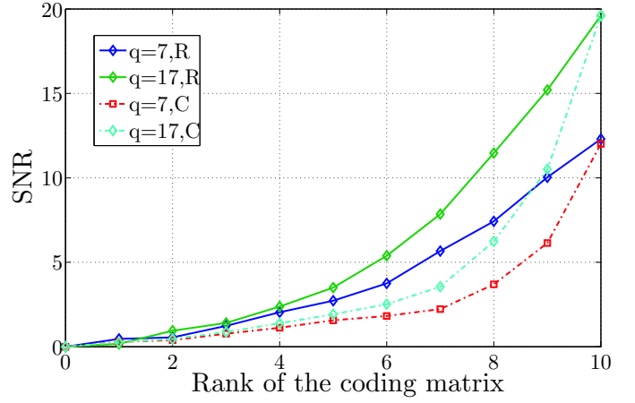
Fig. 2. SNR as a function of the number of linearly independent packets available at the sink for q = 7 and q = 17 , with the proposed approach (R) and with a conventional Gaussian elimination (C)
