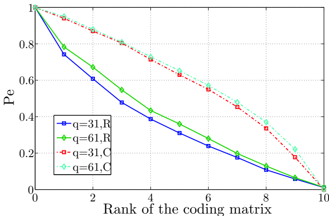
Fig. 5. Proportion of erroneously reconstructed quantized samples as a function of the rank of A sink for q = 31 and q = 61 , with the proposed approach (R) and with a conventional Gaussian elimination (C)
