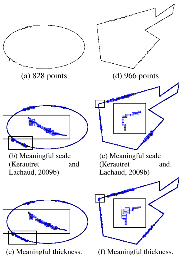
Figure 7: Comparison between meaningful scale (Kerautret and Lachaud, 2009b) (second line) and meaningful thickness (third line). The size of the blue boxes represents for each pixel the obtained meaningful scale or thickness \alpha_\tau . The amount of noise is well evaluated everywhere.
