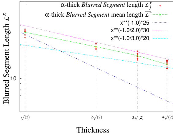
Figure 4: Illustration of the Lengths \mathcal{L}_j^x from the set of \alpha -thick Blurred Segments given from illustration of Fig. 3. The lines of slope -1 , -\frac{1}{2} and -\frac{1}{3} are also given to illustrate the reference constraint of Property 2.
