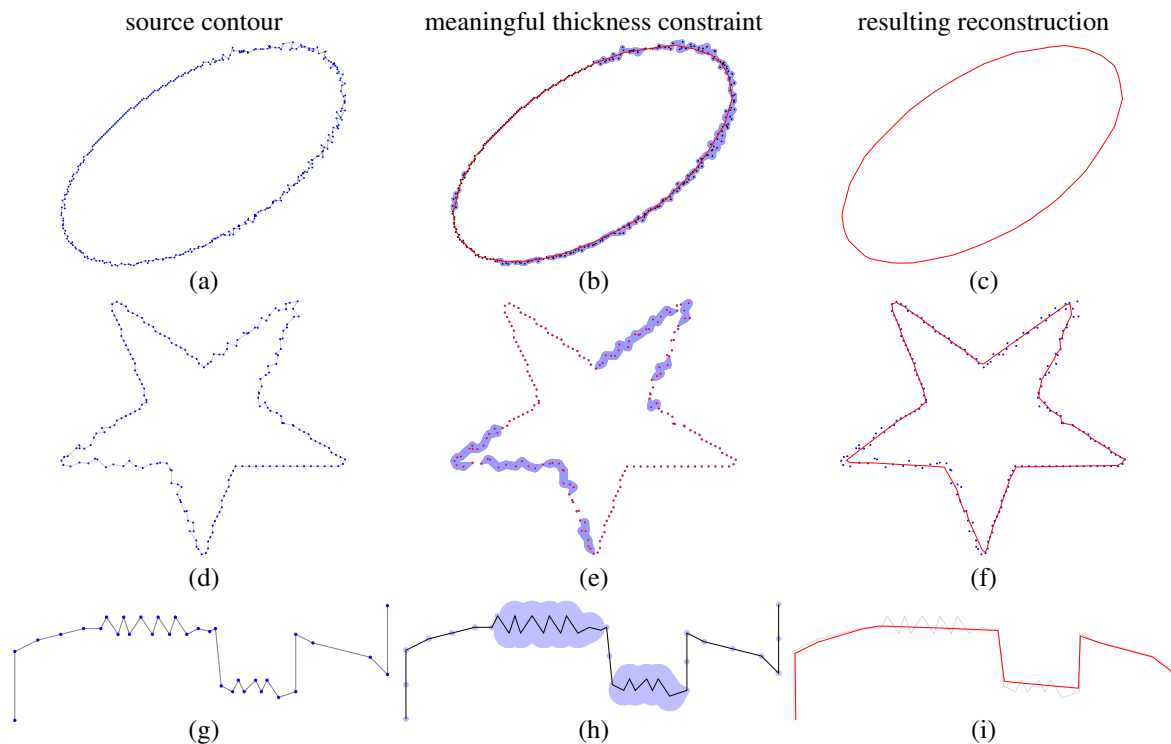
Figure 10: Application of contour smoothing using the meaningful thickness on several shapes. The initial noisy source contour are given in image (a,d,g). The blue areas represent the noise constraints (b,e,h) and the resulting smoothed contour is represented in red on (c,f,i).
