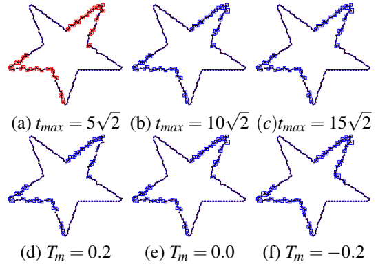
Figure 6: Evaluation of the independence of the meaningful thickness detection from the different parameters. The size of the blue boxes represents for each point the obtained meaningful scale or thickness \alpha_\tau . The first row presents the evaluation by varying the maximal thickness used to define the multi-thickness profile ( t_{max} ). The red color indicates present on image (a) indicates that there exists no meaningful thickness less than t_{max} . The second row shows the stability by the change of the noise threshold parameter T_m .
