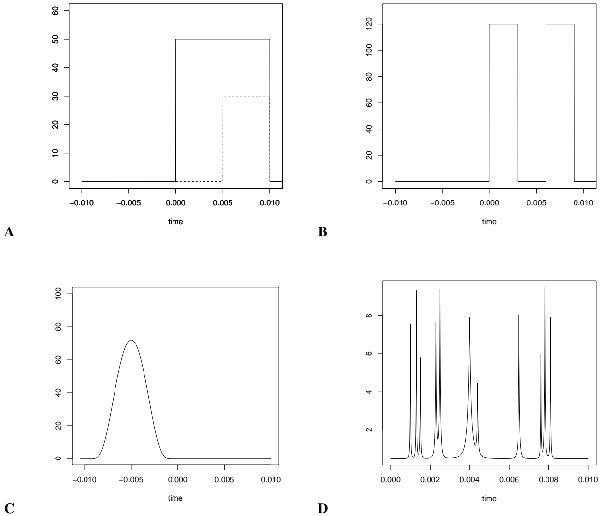
Figure 1: Graphs of alternatives: on Graph A the Echelon functions with h_{50,0} in solid line and h_{30,0.005} in dashed line, on Graph B the Crenel function h_{Crenel} , on Graph C the Bell function h_{Bell} and on Graph D the Bumps function h_{Bumps} .
