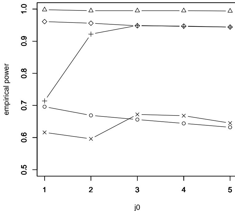
Figure 2: Empirical power associated with our procedure according to j_0 for the alternatives h_{30,0} in \circ - \circ , h_{80,0} in \Delta - \Delta , h_{Crenel} in + - + , h_{Bell} in \times - \times and h_{Bumps} in \diamond - \diamond . The theoretical level is \alpha = 0.05 .
