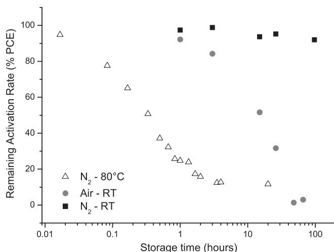
FIG. 3. Remaining Activation Rate as the function of the storage time under N 2 at room temperature (black squares), air at room temperature (grey circles) and N 2 at 80 °C (white triangles).
