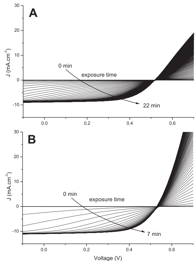
FIG. 1. Current density—voltage curves of solar cells upon light activation. Time delay between curves is 4 s. (a) Devices with pristine TiO_x and (b) devices with TiO_x pre-treated at 180^\circ\text{C} .
