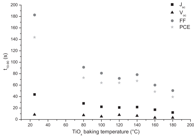
FIG. 2. Evolution of the rising time ( t_{10-90} ) for J_{sc} , V_{oc} , FF and PCE as a function of the baking temperature of TiO_x layer.
