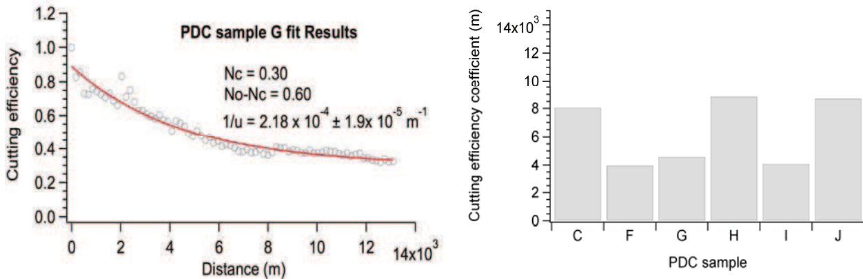
Figure 3. Cutting efficiency vs. distance model for sample G and cutting efficiency coefficients
