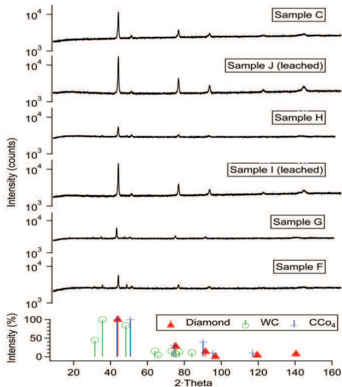
Figure 5. Diffractograms of PDC samples C, F, G, H, I and J classified from low Q (sample F) to high Q (sample C) and calculated stick pattern of diamond, tungsten carbide and cobalt carbide.
