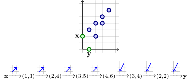
Figure 1. The run \rho labeled by (1, 1)^4(-1, -2)^3 with \text{dir}(\rho) = (\mathbf{x}, \mathbf{y}) .
