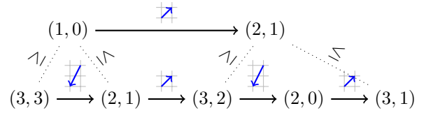
Figure 3. (1, 0)(2, 1) \preceq (3, 3)(2, 1)(3, 2)(2, 0)(3, 1)
