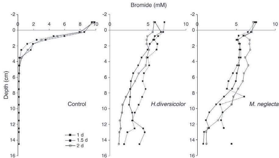
Fig. 4. Bromide pore water profiles (mM) and overlying water concentration ( -1 cm on y-axis) at ca. 1, 1.5 and 2 d of incubation in cores with Hediste diversicolor , Marenzelleria neglecta or no fauna (control).
