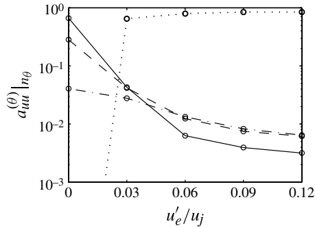
FIGURE 4. Variations with u'_e/u_j of the coefficients a_{uu}^{(\theta)}|_{ln\theta} obtained from the cross-correlation functions \mathcal{R}_{uu}^{(\theta)} of velocity u'_z at r = r_0 and z = 0.4r_0 : —, n_\theta = 0 ; ---, n_\theta = 1 ; - · - ·, n_\theta = 2 ; ·····, sum for n_\theta \geq 21 .
