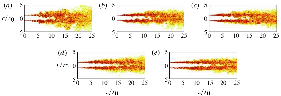
FIGURE 19. (Colour online) Snapshots in the (z, r) plane of vorticity norm |\omega| in the full jets up to z = 25r_0 : (a) Jet0%, (b) Jet3%, (c) Jet6%, (d) Jet9%, (e) Jet12%. The colour scale ranges up to the level of 5u_j/r_0 .
