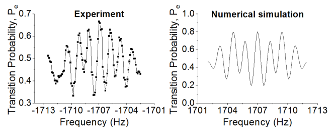
FIG. 12: Fringe pattern of the accordion interferometer, for Raman pulses of \tau_R = 140 ms and separation time of T = 65 ms. Left: measured. Right: calculated. Resonant frequency inhomogeneities of about \sigma_{RDLS} = 2.5 Hz centered at \nu_{RDLS} = 0 Hz.
