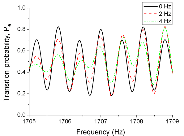
FIG. 15: (Color online) Distortion of the central fringe of the \Delta m = +3 intersite transition. The different interferometer fringe patterns are numerically calculated for different value of the mean RDLS \nu_{RDLS} , and for a \tau_R = 140 ms, T = 175 ms, \sigma_{RDLS} = 2.5 Hz. The central fringe of the interferometer pattern is situated at -1707 Hz.
