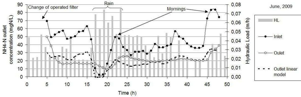
Fig. 1. NH 4 -N concentration during two successive 24-h flow composite samples, 100% RFR (June, 2009)
