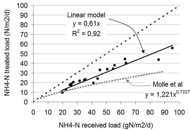
Fig. 2. Treated NH 4 -N, 100% RFR and C in > 40 mgNH 4 -N.L -1 (June, 2009)
