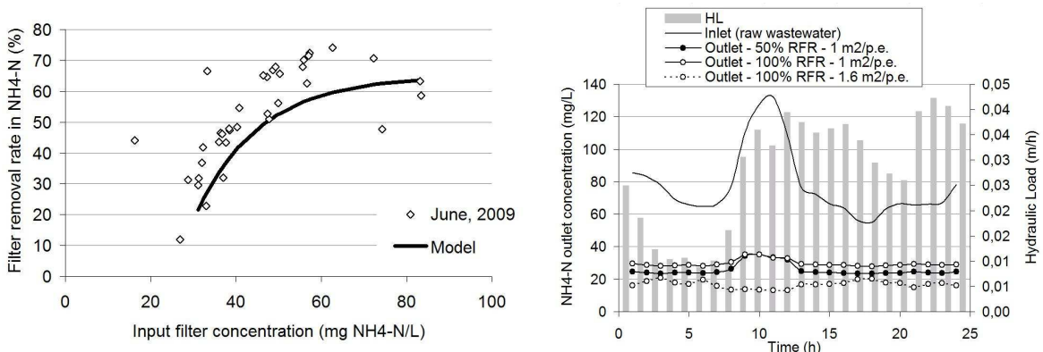
Fig. 3. 3a), Schedule nitrification yields linked to NH 4 -N inlet concentrations and, 3b), Evolution of the theoretical outlet NH 4 -N concentrations according to different design and RFR conditions
