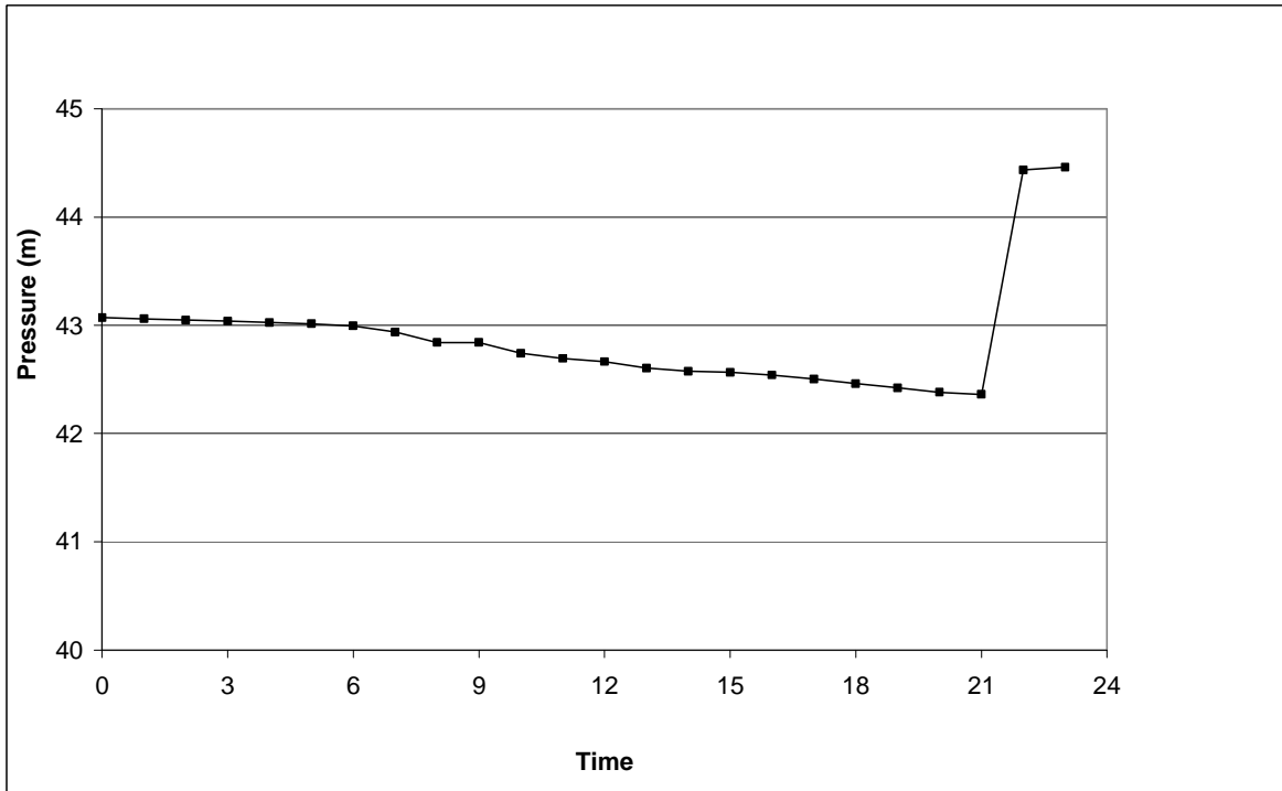
Figure 1 RMMS De la Réole. “Hydraulic model” method. Dynamic hourly pressure of DMA S1 over 24 hours
