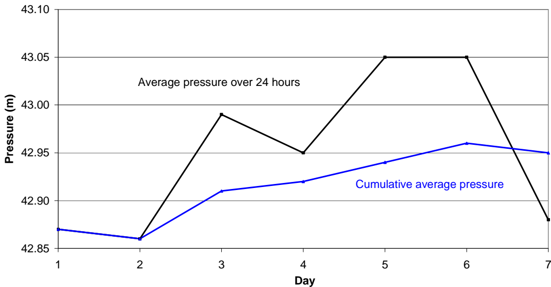
Figure 2 RMMS De la Réole. “Hydraulic model” method. Average pressures of DMA S1 over a week
