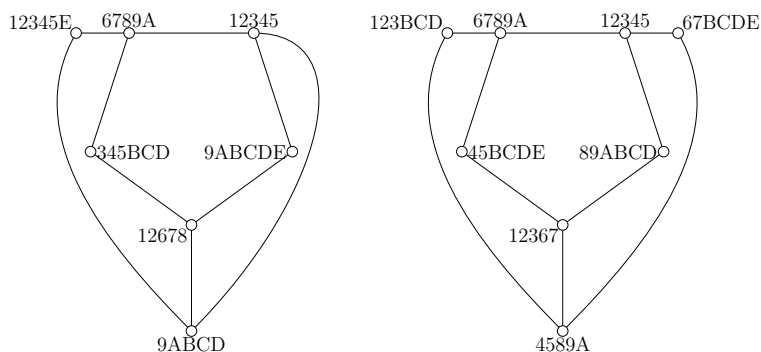
Figure 9: Configurations from Lemma 3.12.
