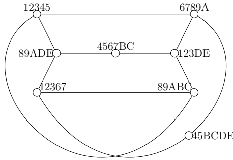
Figure 10: A configuration from Lemma 3.14.
