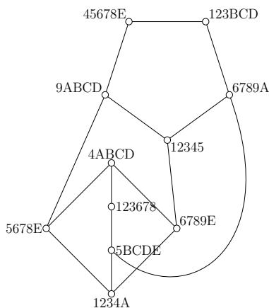
Figure 7: Configuration from Lemma 3.9.
