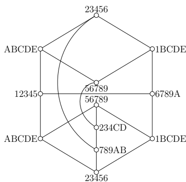
Figure 8: A configuration from Lemma 3.10.
