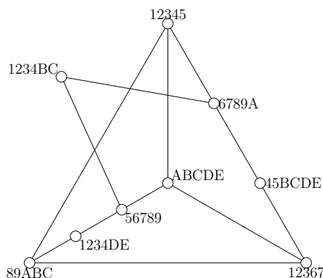
Figure 5: A dangerous induced subgraph with two safe vertices.
