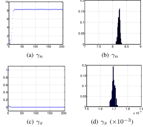
Fig. 1. Chains and histograms of hyperparameters \gamma_n and \gamma_x .
