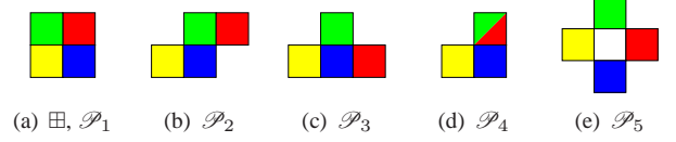
Fig. 3: (a) Configuration forbidden in well-composed images (see Th. 3). (a,b,c) Configurations forbidden in regular images (see Def. 9). (These configurations are given up to \pi/2 rotations, symmetries and values inversion.)
