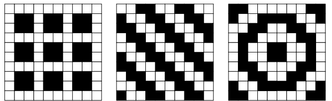
Fig. 6: Well-composed images that cannot be modified (without a super-resolution approach) to fulfil regularity requirements, due to fine texture effects.
