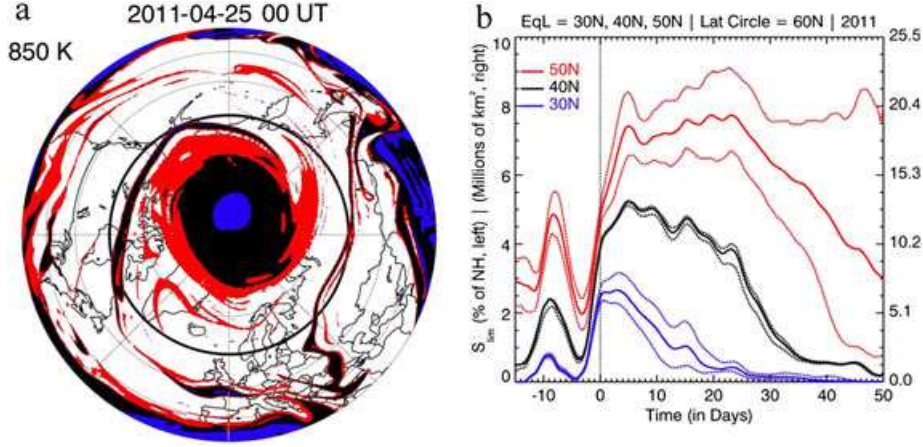
Figure 4. (a) MIMOSA PV fields with values lower than PV_{lim} for \Phi_{eq,lim} = 30^\circ\text{N} , 40^\circ\text{N} and 50^\circ\text{N} (in blue, black and red, respectively) on 25 April 2011 at 850 K. (b) Time evolution of the spatial extent S_{lim} northward of 60^\circ\text{N} obtained for \Phi_{eq,lim} = 30^\circ\text{N} , 40^\circ\text{N} and 50^\circ\text{N} , respectively, at 850 K. Spatial extent is expressed either in %NH (left axis) and in millions squared kilometers (right axis). In Figure 4b, the vertical dashed (solid) line denotes the turnover date (see text).
