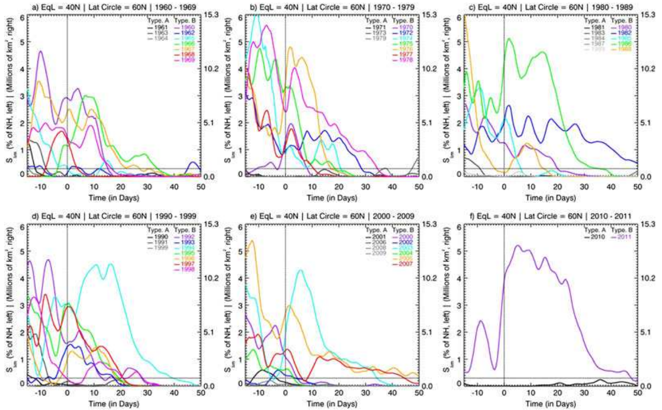
Figure 5. Time evolution of the spatial extent S_{lim} during the (a) 1960s, (b) 1970s, (c) 1980s, (d) 1990s, (e) 2000s, and (f) 2010s, computed northward of 60^{\circ}\text{N} and for \Phi_{eq,lim} = 40^{\circ}\text{N} . The horizontal dashed line at 0.3%NHA denotes the climatological confidence interval. Type-A years are shown in black or gray, while Type-B years are shown in color.
