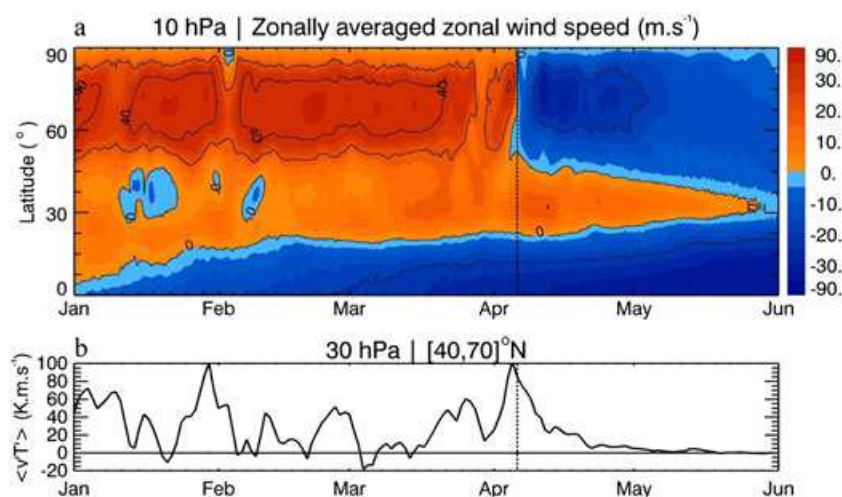
Figure 1. (a) Time series of the ERA-Interim zonal-mean zonal wind (in m/s) from 1 January to 1 June 2011 at 10 hPa over the Northern Hemisphere (b) zonal-mean meridional eddy heat flux averaged over the [40,70]^{\circ}\text{N} latitude range at 30 hPa. The vertical dashed lines correspond to the turnover date of April 6.
