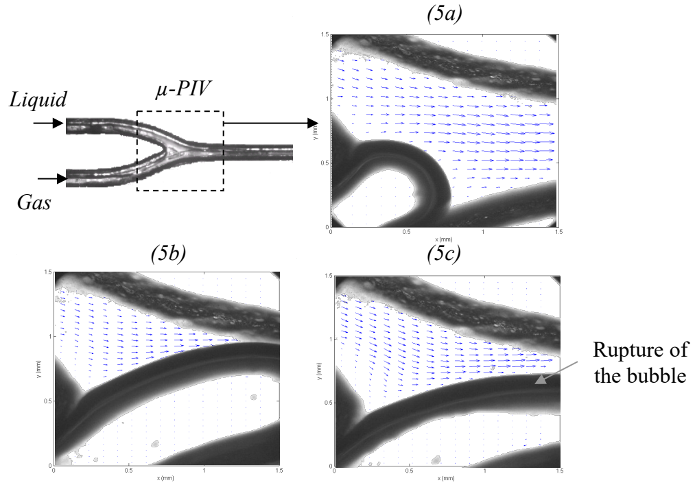
Figure 5. Velocity Flow fields around a forming air bubble in a Y-junction of 800 \mu m in water + 0.15% (wt) SDS, Q_1 = 10^{-7} \text{ m}^3/\text{s} ( v_1 = 0.2 \text{ m/s} ), \sigma = 40 \text{ mN/m} .
