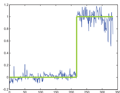
Figure 6: Membership degree functions estimated by PLS for the 335 samples on the abscissa: sample number (samples are sorted by class) in green: targeted binary values
