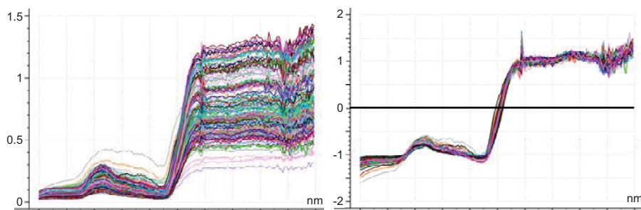
Figure 4: SNV transformation applied to a set of wheat spectra
