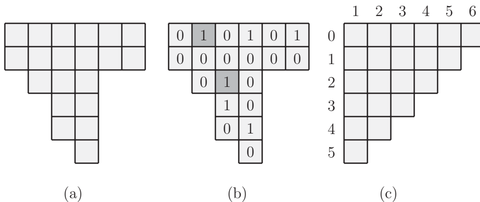
FIGURE 18. (a) a stack polyomino of shape (2, 3, 5, 6, 2, 2) ; (b) a filling of this polyomino, with a shaded 2-diagonal; (c) the polyomino A_7 .
