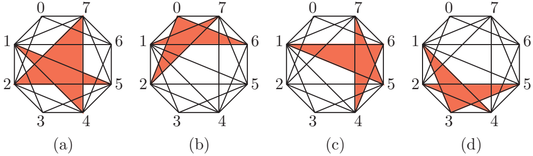
FIGURE 8. The four 2-stars in the 2-triangulation of the octagon of Figure 2.
