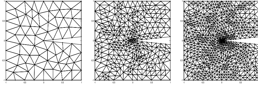
FIG. 7.6. Mesh refinements 1, 7 and 10 for the singular solution, \lambda = 10^4 .
