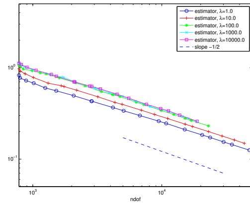
FIG. 7.7. Estimator convergence rate in ndof for the singular solution, \lambda from 1 to 10^4 .
