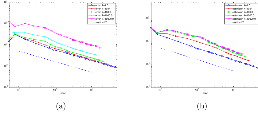
FIG. 7.4. Error (a) and Estimator (b) convergence rates in ndof for the regular solution, n = 25 , \lambda from 1 to 10^4 .
