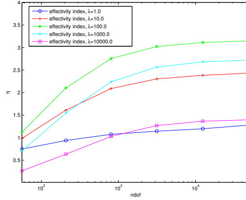
FIG. 7.2. Effectivity index I_{eff} for the regular solution, n = 2 , \lambda from 1 to 10^4 .
