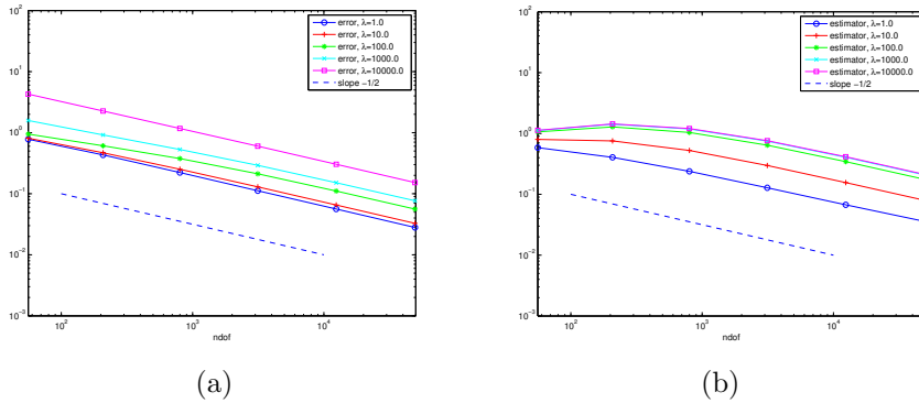
FIG. 7.1. Error (a) and Estimator (b) convergence rates in ndof for the regular solution, n = 2 , \lambda from 1 to 10^4 .
