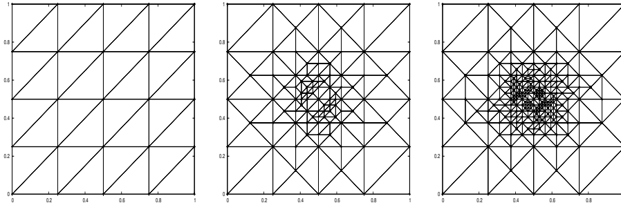
FIG. 7.3. Mesh refinements 1, 4 and 7 for the regular solution, n = 25 , \lambda = 10^4 .
