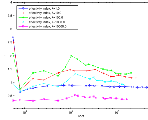
FIG. 7.5. Effectivity index I_{eff} for the regular solution, n = 25 , \lambda from 1 to 10^4 .
