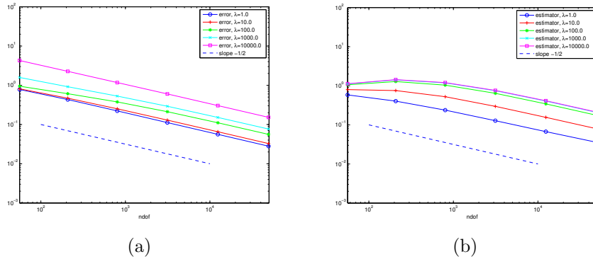
FIG. 7.1. Error (a) and Estimator (b) convergence rates in ndof for the regular solution, n = 2 , \lambda from 1 to 10^4 .
