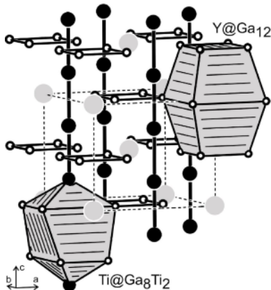
Fig. 1. The crystal structure of \text{YTi}_2\text{Ga}_4 . Yttrium, titanium and gallium atoms are drawn as medium grey, black filled and open circles, respectively. The coordination polyhedra around the yttrium and titanium atoms as well as the titanium chains and the \text{Ga}_4 squares are emphasized.
