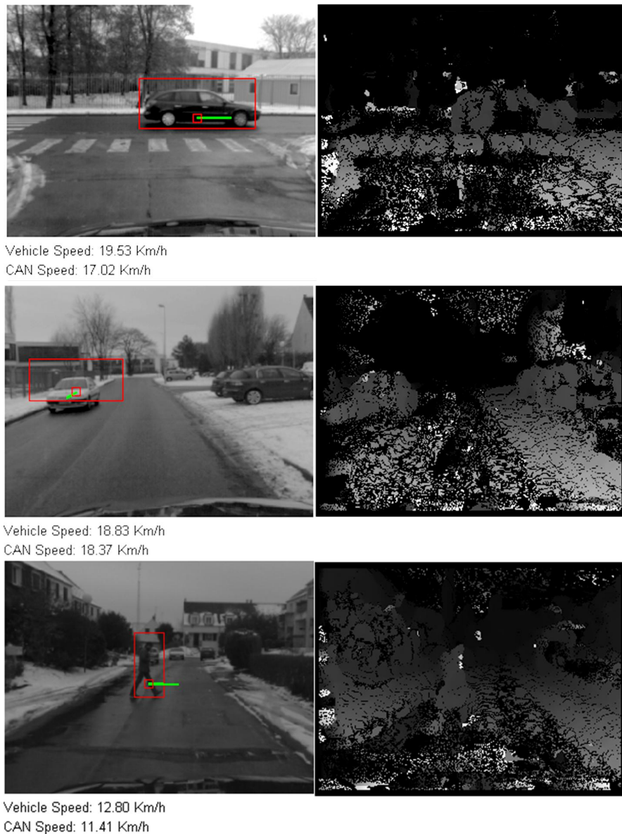
Fig. 25 Confirmed objects. The top figure illustrates the visual confirmation of a highly dynamic object (Scenario B in Fig. 23). The middle figure shows a vehicle having just turned. Here the ROI is delocalized because of pitch changes, given that the ego-vehicle is accelerating (Scenario C in Fig. 23). The bottom figure shows the confirmed pedestrian when crossing the road in Scenario E (Fig. 23)
