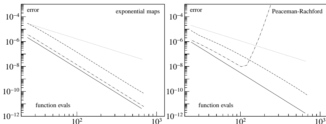
Fig. 4.3 Plot: Nonlinear case – Error ( L^2 norm at time T ) versus number of evaluations of the basic method \Phi_h . Strang splitting (dotted lines), “quadruple jump” composition method \Psi_h^{(4)} (solid line), extrapolation method (4.2) (dashed-dotted line), extrapolation method (4.3) (dashed lines). Left picture: Basic method is the Strang splitting with exponential maps (2.3). Right picture: Peaceman-Rachford formula (2.4).
