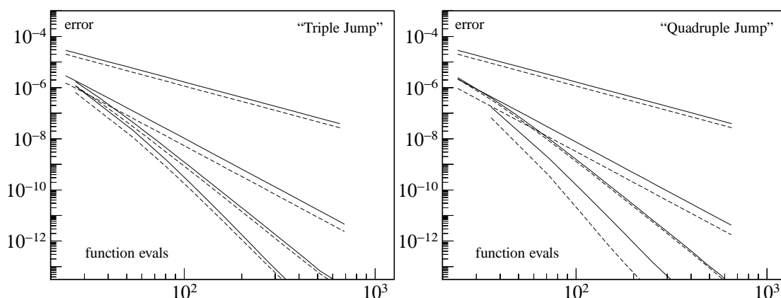
Fig. 4.2 Plot: Nonlinear case – Error ( L^2 norm at time T ) of composition methods versus number of evaluations of the basic method \Phi_h . Left picture: “triple jump” composition methods \widetilde{\Phi}_h^{(p)} , p = 2, 4, 6, 8 . Right picture: “quadruple jump” composition methods \Psi_h^{(p)} , p = 2, 4, 6, 8 . For all these pictures, solid lines: basic method is the Strang splitting with exponential maps (2.3) – dashed lines: basic method is the Peaceman-Rachford formula (2.4).
