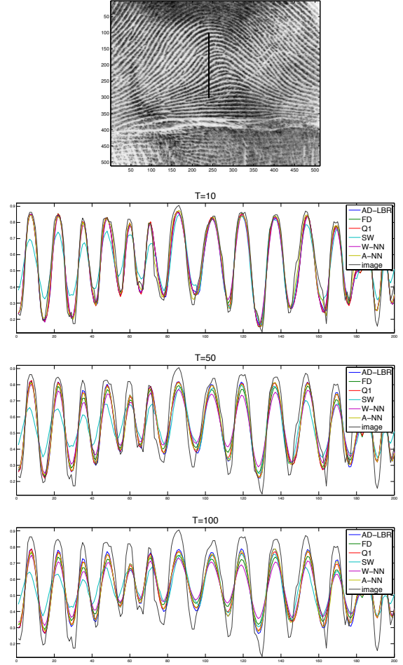
Figure 13: Evolution under CED of a section of the fingerprint image. The ridges in the evolved image are higher, and the valleys are deeper, with AD-LBR than with the other schemes. This illustrates the fact that AD-LBR, respecting the continuous PDE, diffuses more along the structure and less in the orthogonal direction. From top to bottom: location of the section of the image; section at T = 10 ; section at T = 50 ; section at T = 100 .
